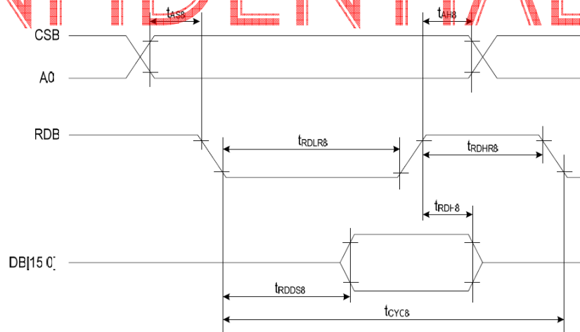
( Read Timing )
